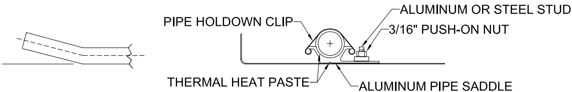
VIEW B-B
